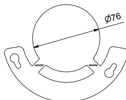
3711308 - Large Restrictor D76
